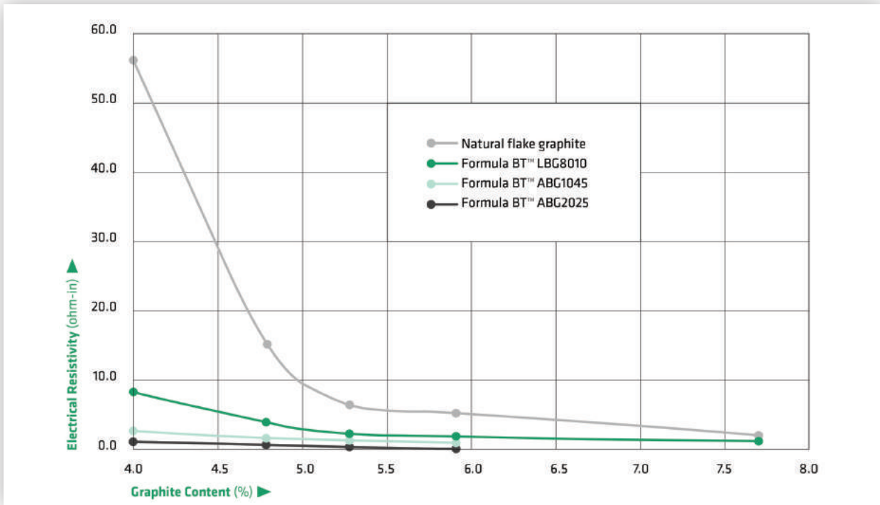
Electrical Resistivity of MnO 2 /Graphite Mix as a Function of the Graphite Content
