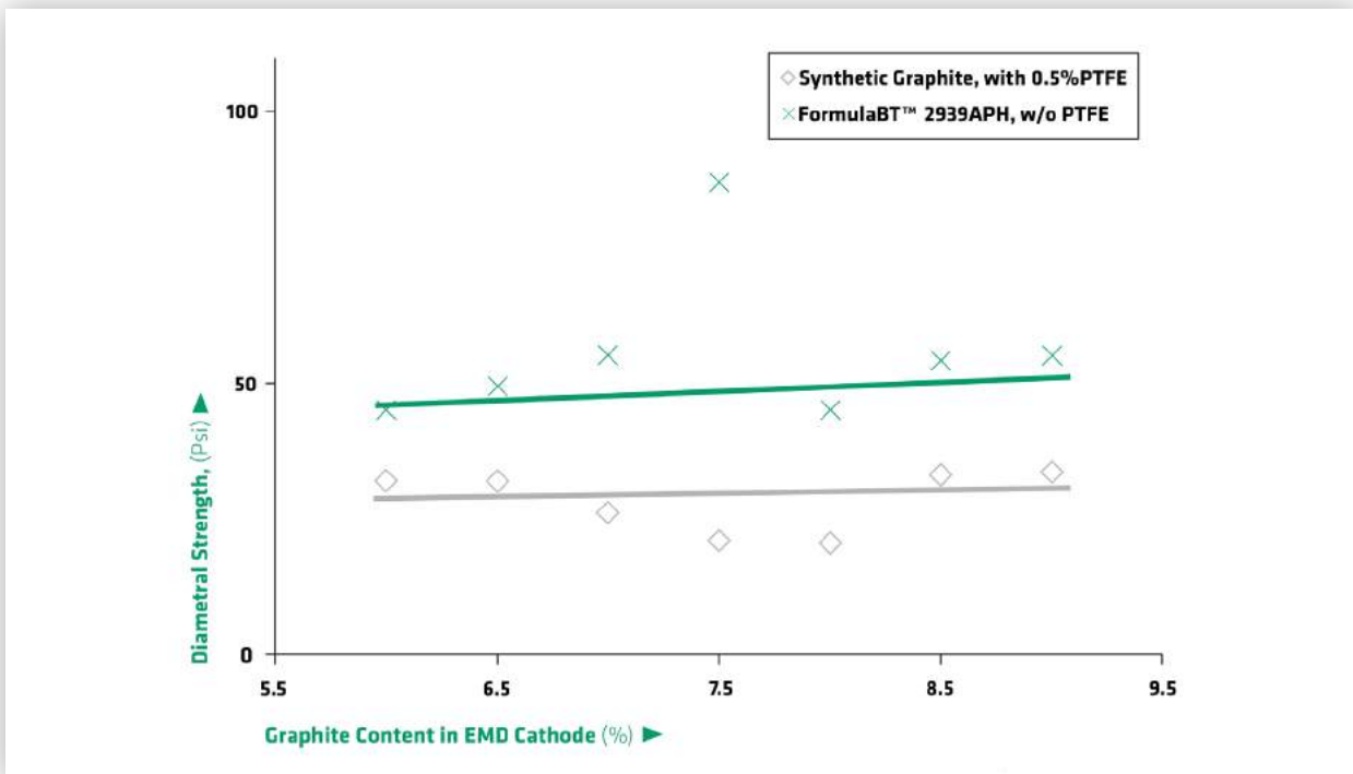
Mechanical Strength of MnO 2 /Graphite Tablets
